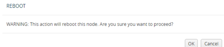
Figure 22 Reboot Dialog
