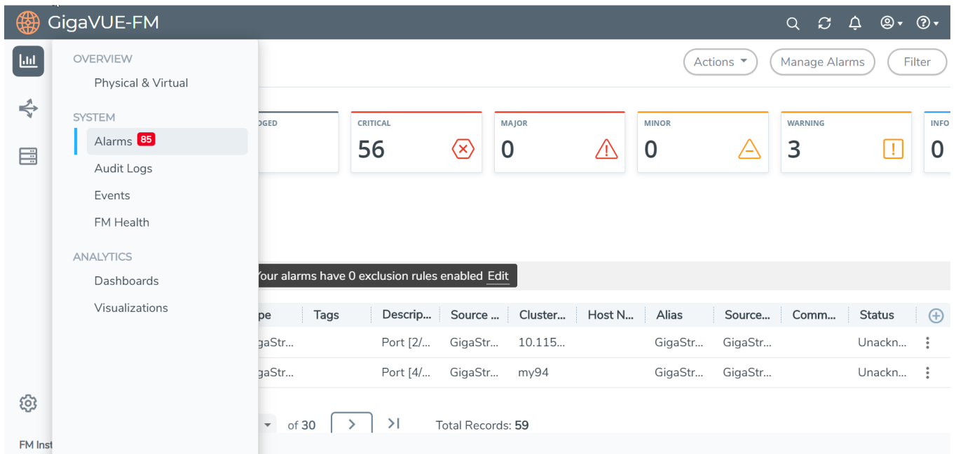
Figure 13 Alarms
